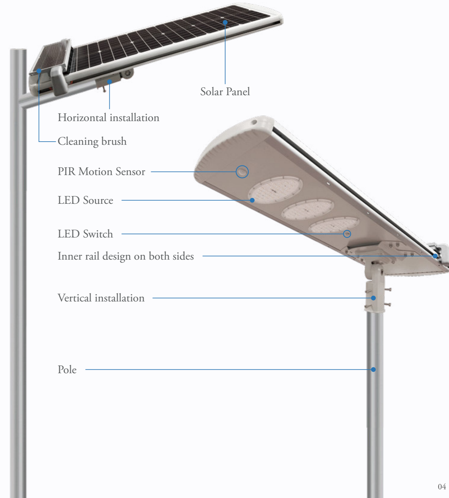
Dust off : Clean panels, faster power generation.
